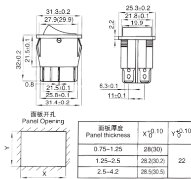
KCD4-202/4PN
