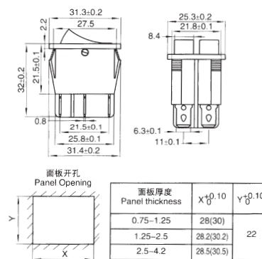
KCD3-202NM
